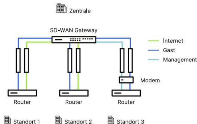
Abbildung 9: Advanced Routing and Forwarding (ARF).
